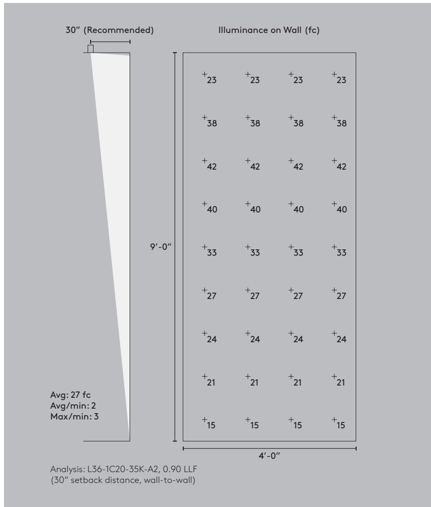
The A2 - LMO Asymmetric 20° Wall Washer provides high quality optical performance, translating into an even distribution of light on the wall.
