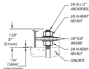
BOLT CIRCLE DETAIL (NOT TO SCALE)
