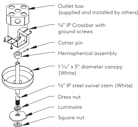
L1DI Swivel Stem (S) Suspension Detail (feed wires through stem supplied by others)
