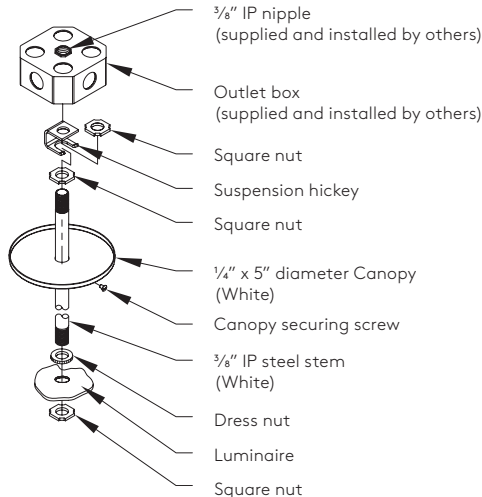
L1DI Rigid Stem (RS) Suspension Detail (feed wires through stem supplied by others)
