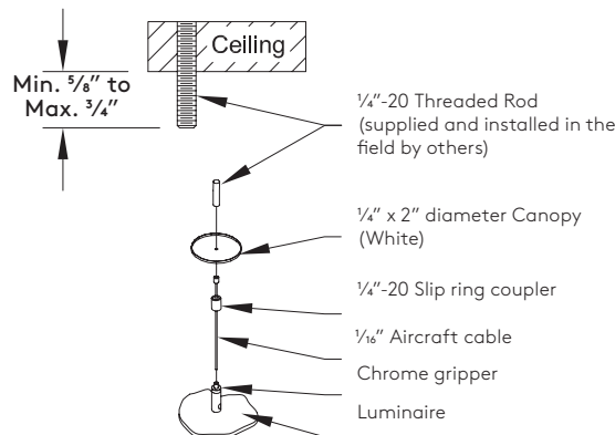
L10 Cable (C) Suspension Detail (Non-Feed location(s) only)
