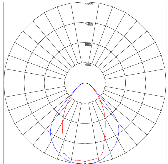
Maximum Candela = 1959 Located At Horizontal Angle = 0, Vertical Angle = 1 # 1 - Vertical Plane Through Horizontal Angles (90 - 270) # 2 - Vertical Plane Through Horizontal Angles (0 - 180)
