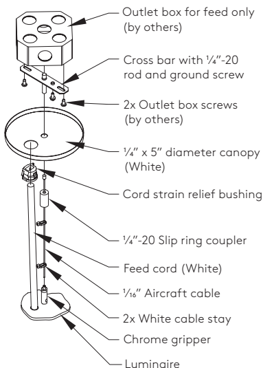
L10 Cable (C) Suspension Detail (Feed location(s) only)
