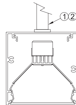
Stem Mounting (S and RS)
