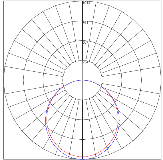
Maximum Candela = 1014 Located At Horizontal Angle = 0, Vertical Angle = -5 # 1 - Vertical Plane Through Horizontal Angles (90 - 270) # 2 - Vertical Plane Through Horizontal Angles (0 - 180)
